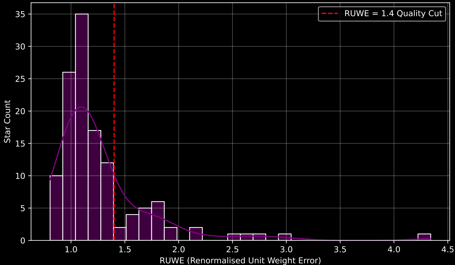
GALAH DR4 Field [6596] RUWE Distribution (n= 126)
