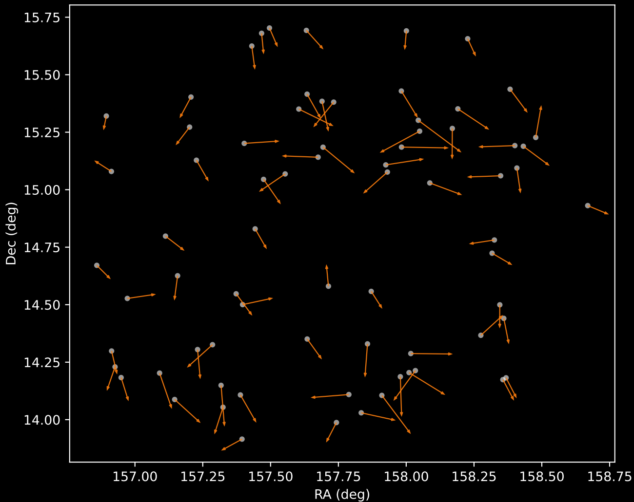
GALAH DR4 Cluster 2 Proper Motion Vectors (n=73)
