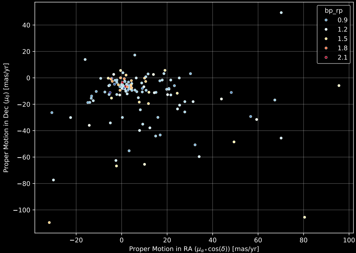
GALAH DR4 Field: [6596] Proper Motion Diagram (n= 131)
