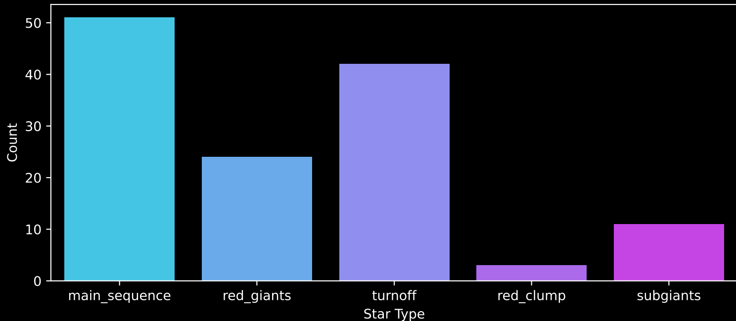
GALAH DR4 Field: [6596] Count plot of Star Type
